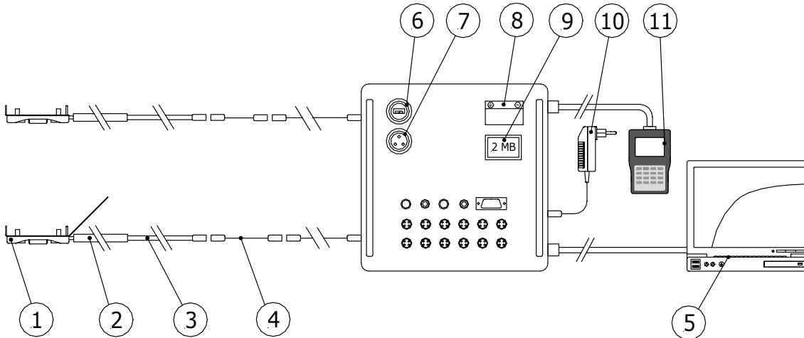
Figure 1 Schematic overview of the measurement system; (1) HF01 sensor with magnet frame, (2) HF01 cable metal insulated with silicone sleeve. (3) HF01 cable Teflon. (4) Teflon extension cables with 2 connectors. (5) PC or laptop (not part of the system). (6) USB connector for connection to PC or laptop. (7) connector for charger. (8) battery. (9) system memory. (10) charger (110/220 VAC). (11) Keyboard Display (LCD Display). Items 6 to 11 are the MCU.
