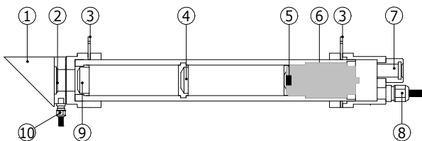
Figure 1: DR01 pyrhelimeter: (1) protection cap, (2) window with heater, (3) sight, (5) sensor, (7) humidity indicator, (10) cable for heater
