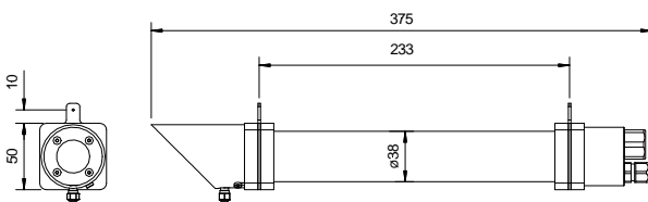
Figure 2: DR01 dimensions
